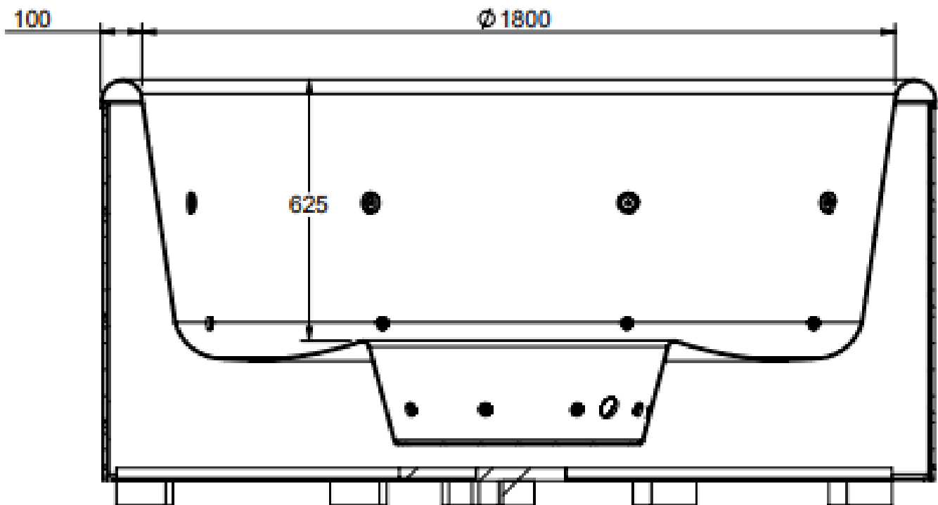
SECTION E-E
